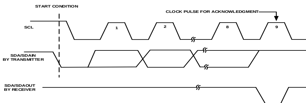
Figure 8 Acknowledge
