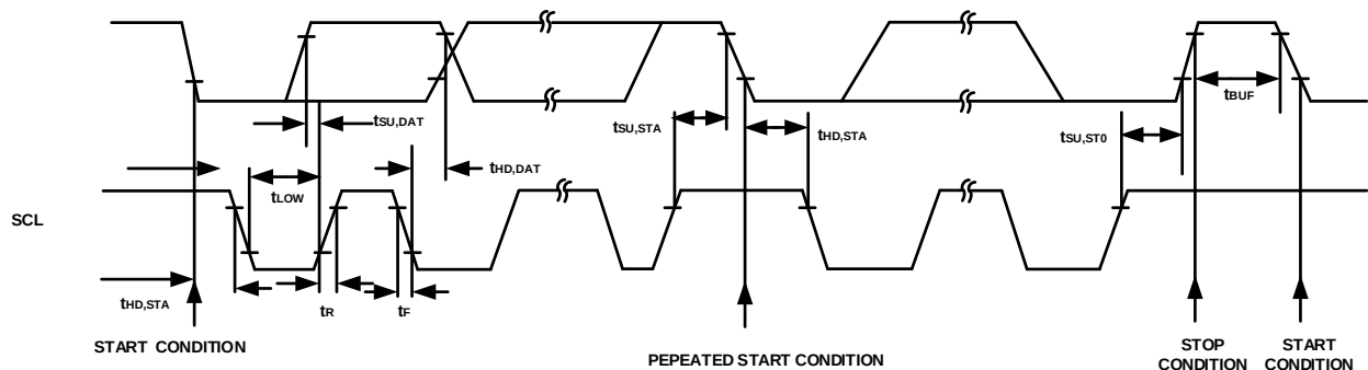
Figure 5 Serial Interface Timing Details
