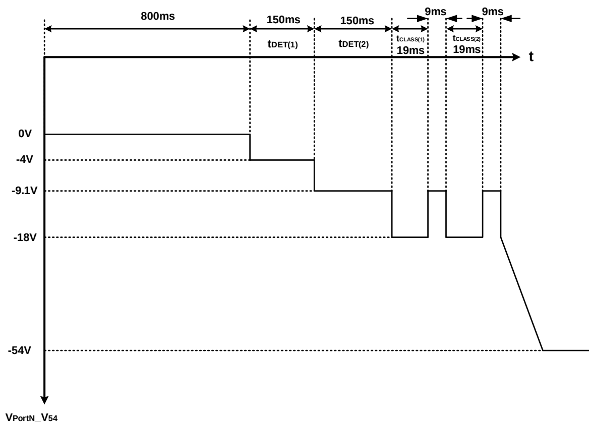
Figure 2. Detection, 2-Event Classification, and Port Power-Up Sequence
