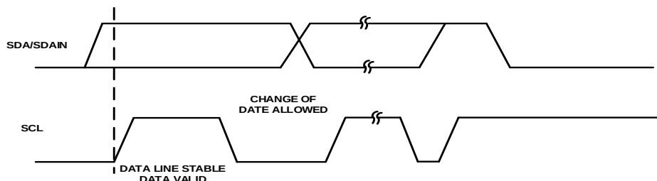
Figure 7 Bit Transfer
