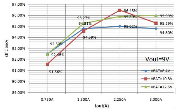
Fig. 4 Efficiency
