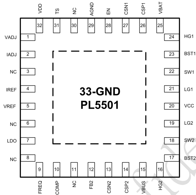
Fig. 2 Pin-Function (QFN4X4-32)
