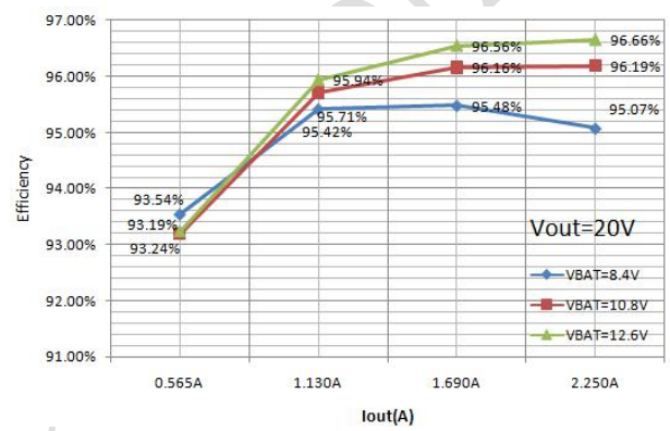
Fig. 6 Efficiency
