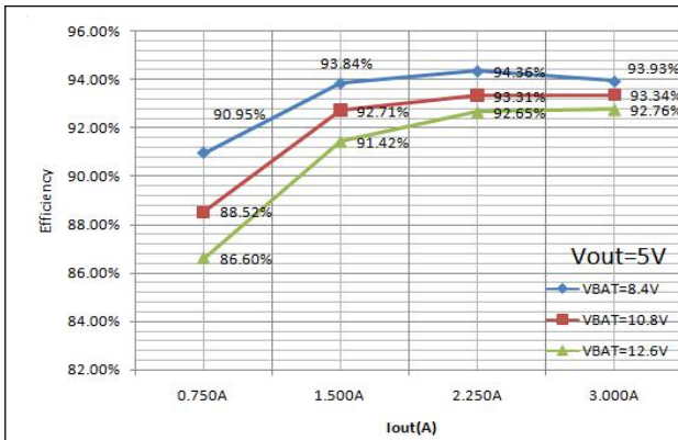
Fig. 3 Efficiency
