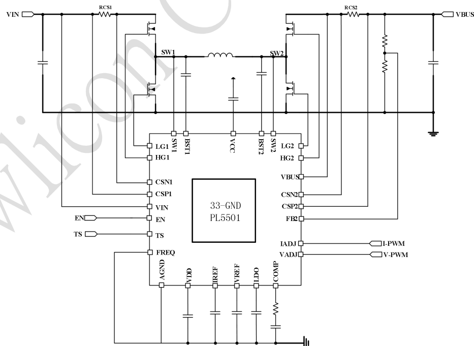
Fig. 1 Application Schematic
