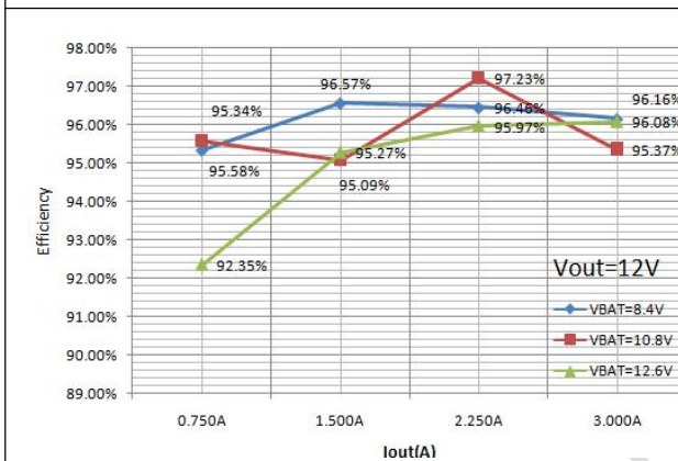
Fig. 5 Efficiency
