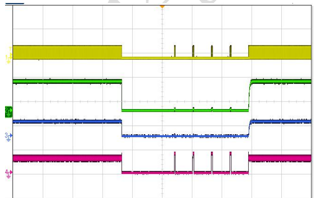
Fig.28 Short Circuit waveform
