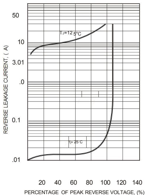
FIG.4-TYPICAL REVERSE CHARACTERISTICS
