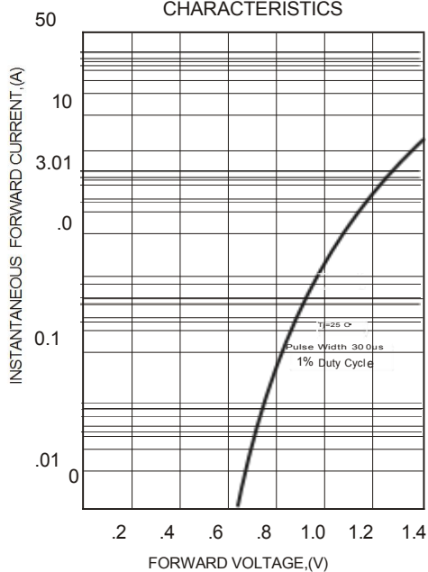
FIG.3-TYPICAL FORWARD CHARACTERISTICS
