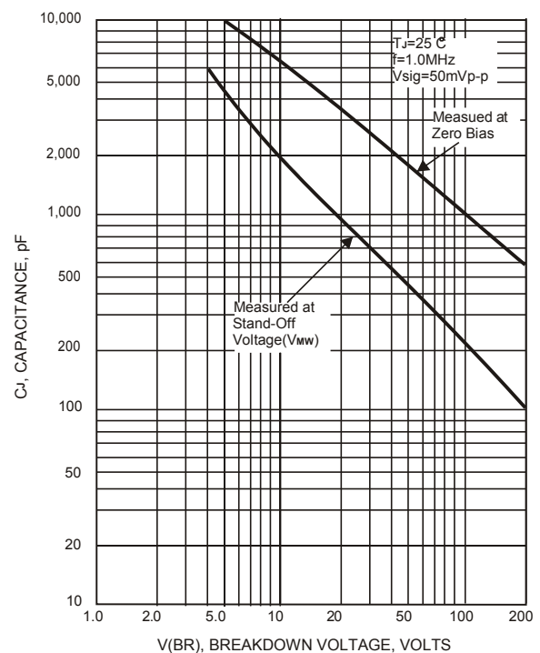
FIG.4-TYPICAL JUNCTION CAPACITANCE
