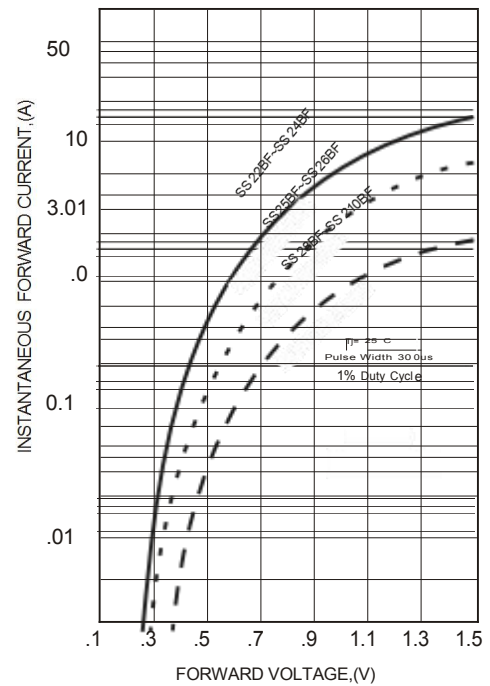
FIG.2-TYPICAL FORWARD CHARACTERISTICS
