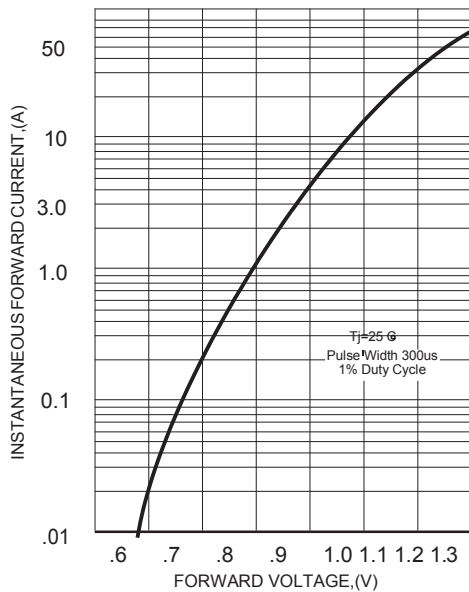
FIG.1-TYPICAL FORWARD CHARACTERISTICS
