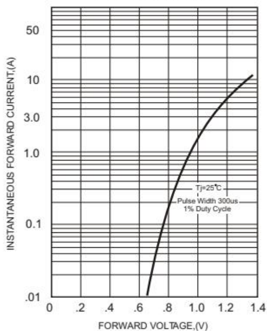
FIG.3-TYPICAL FORWARD CHARACTERISTICS
