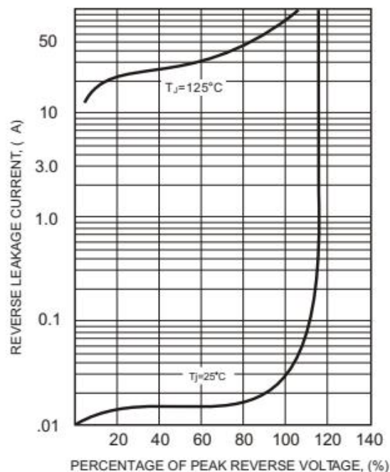
FIG.4-TYPICAL REVERSE CHARACTERISTICS
