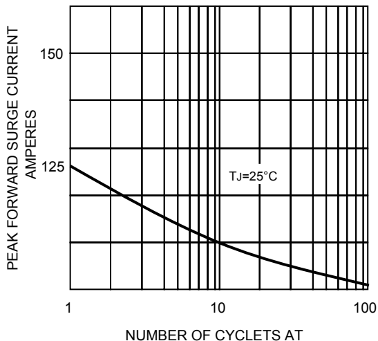
FIG.1-MAXIMUM FORWARD SURGE
