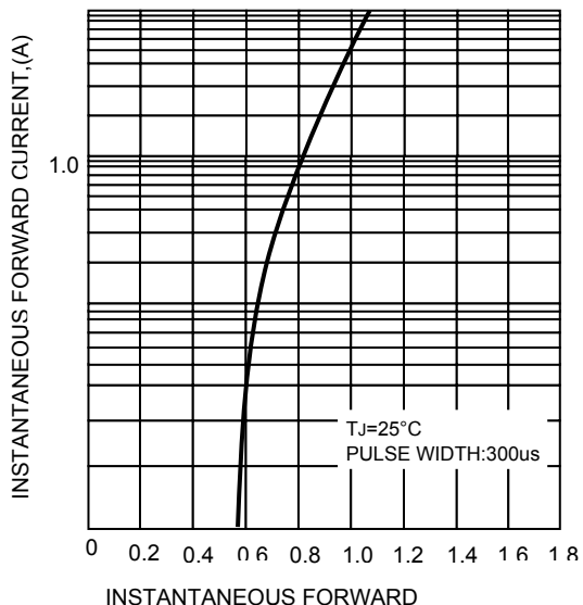
FIG.4-TYPICAL FORWARD
