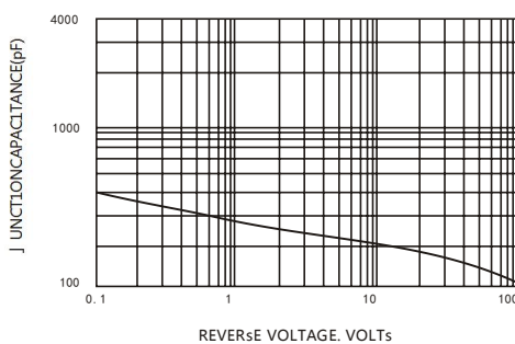
FIG.5-TYPICAL JUNCTION CAPACITANCE
