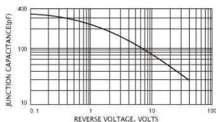
FIG.5-TYPICAL JUNCTION CAPACITANCE
