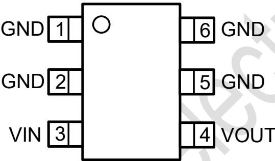
SOT23-6 (Top View)
