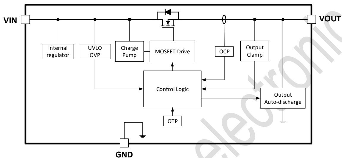
Figure 2. TMI6401 Block Diagram
