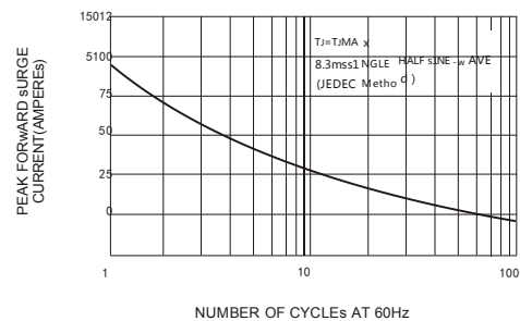
FIG.2-MAXIMUM NON-REPEATABLE PEAK FORWARD SURGE CURRENT
