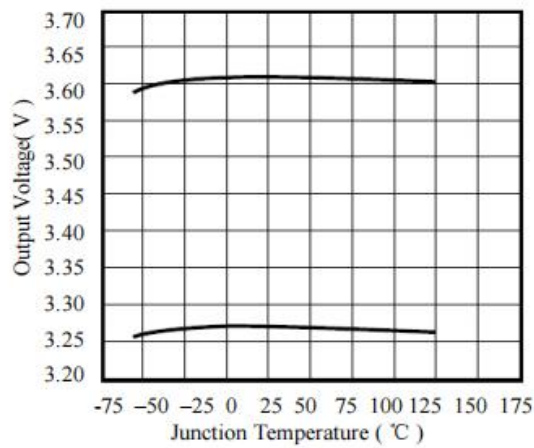
Figure 6. Output Voltage VS. Temperature
