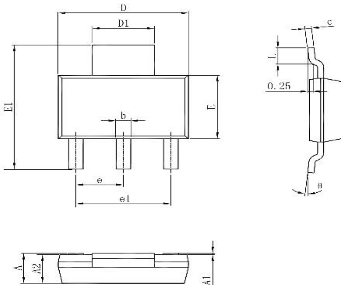
SOT-223 PACKAGE OUTLINE DIMENSIONS
