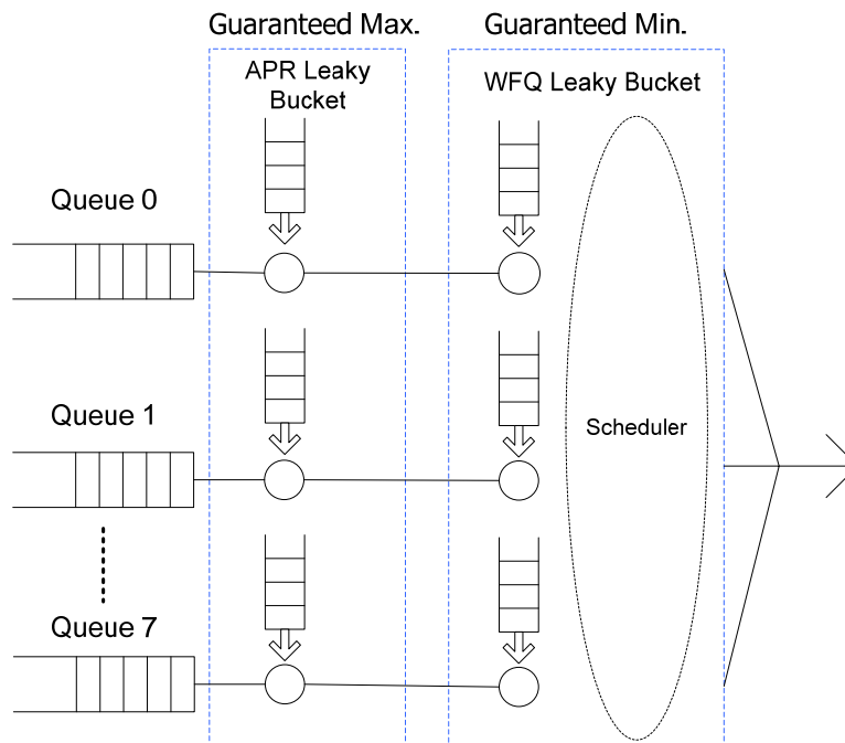
Figure 7. RTL8367S MAX-MIN Scheduling Diagram
