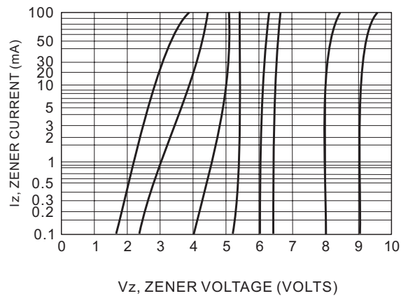
Fig.7 V_z = 6.8 thru 10 Volts
