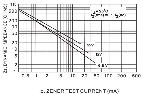
Fig.4 Zener impedance v.s. zener current
