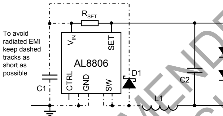
Figure 6 PCB Layout
