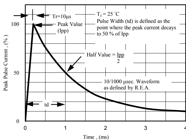
Fig. 5 - Pulse Waveform
