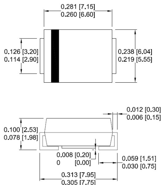
SMC/ DO-214AB
