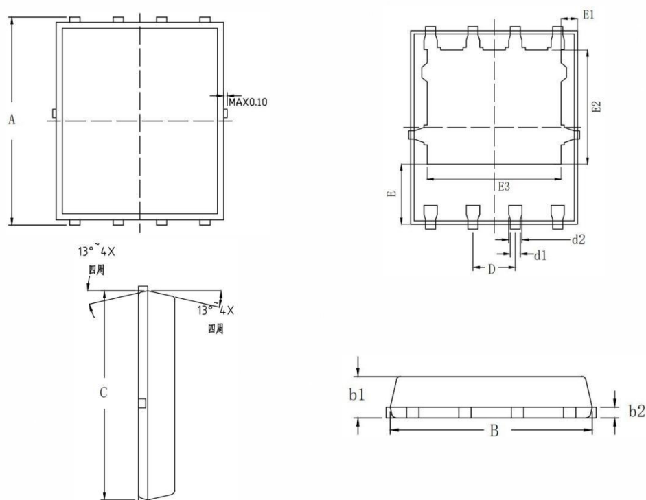
COMMON DIMENSION(MM)
