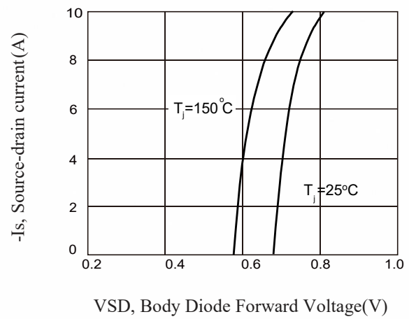
Fig.8 Typical Source-Drain Diode Forward Voltage
