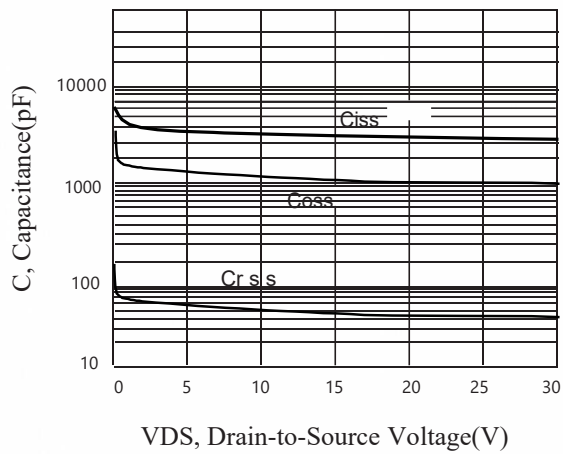
Fig.7 Capacitance
