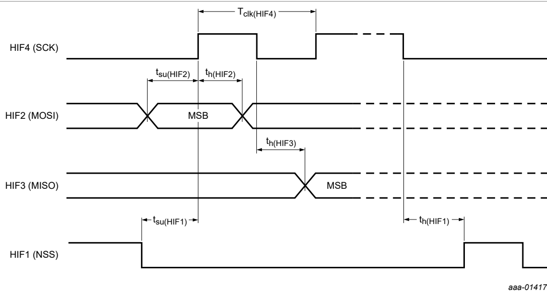
Figure 34. SPI-bus timing diagram
