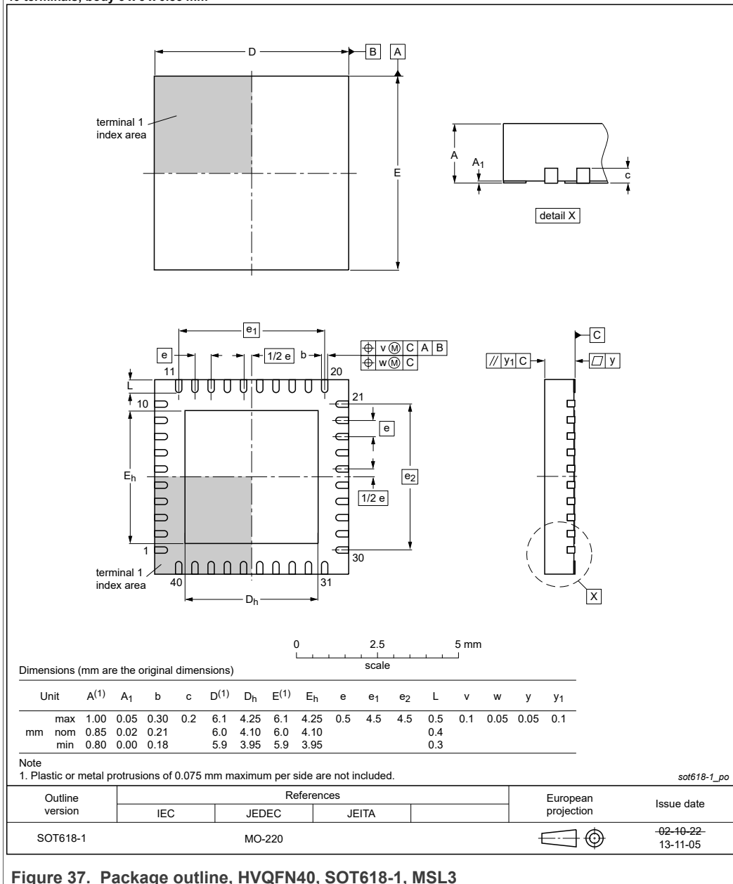
Figure 37. Package outline, HVQFN40, SOT618-1, MSL3
