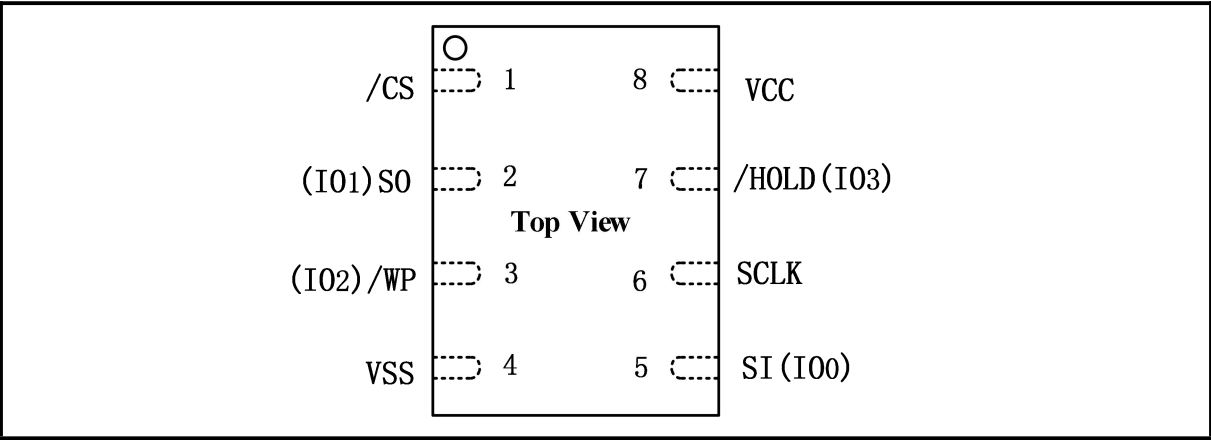
Figure 3. Pin Configuration WSON8 5*6mm,USON8 4*3mm and LGA8 2*3mm
