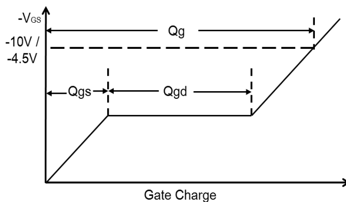
Fig.10 Gate Charge Waveform
